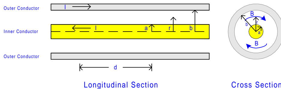
Figure 1: Toroid & Coaxial Cable Inductance Formulas
