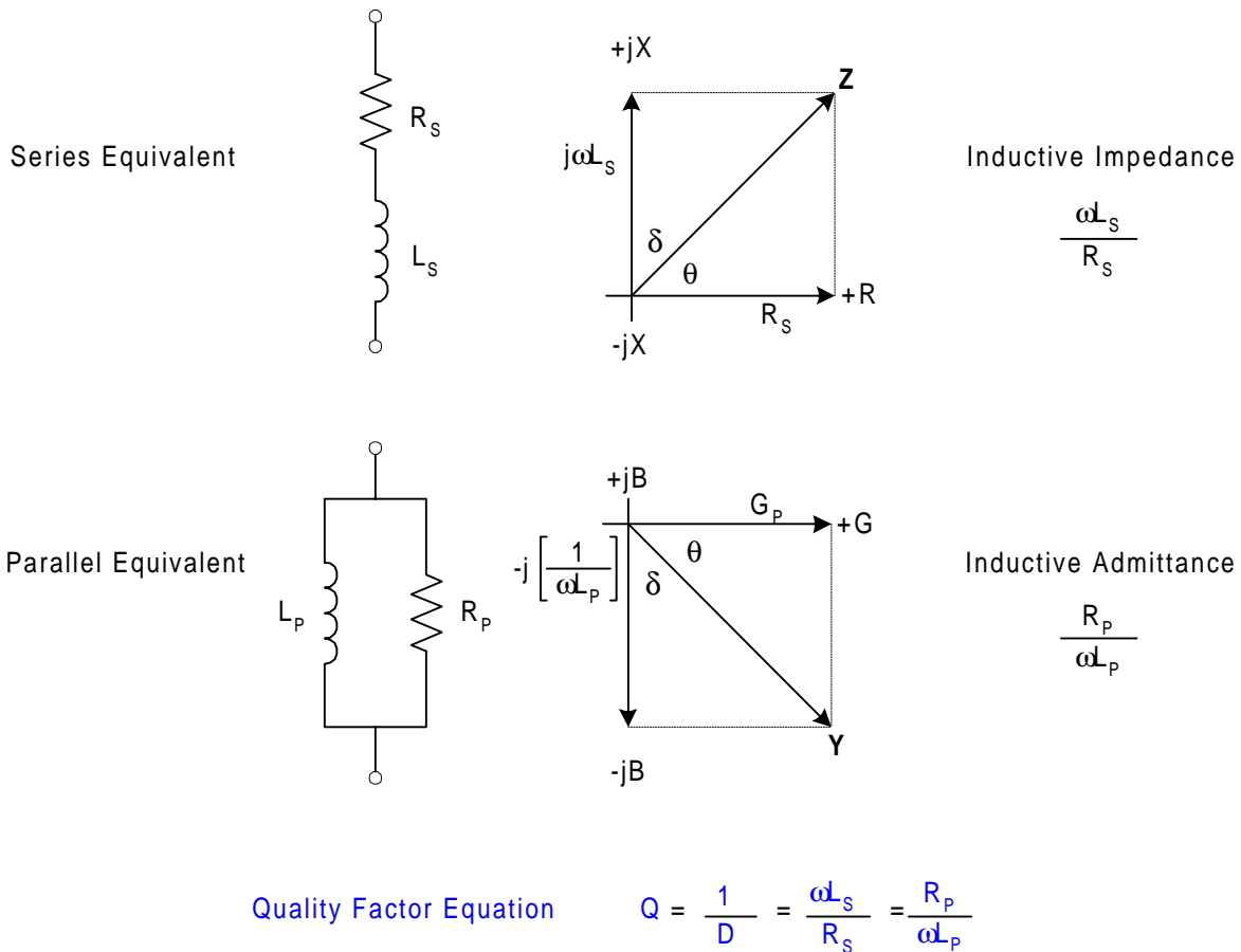
Figure 2: Quality Factor Equation
