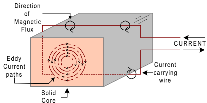
Figure 4: Eddy Currents induced in a solid iron core
